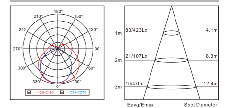
16W-LPTL10D04-2
